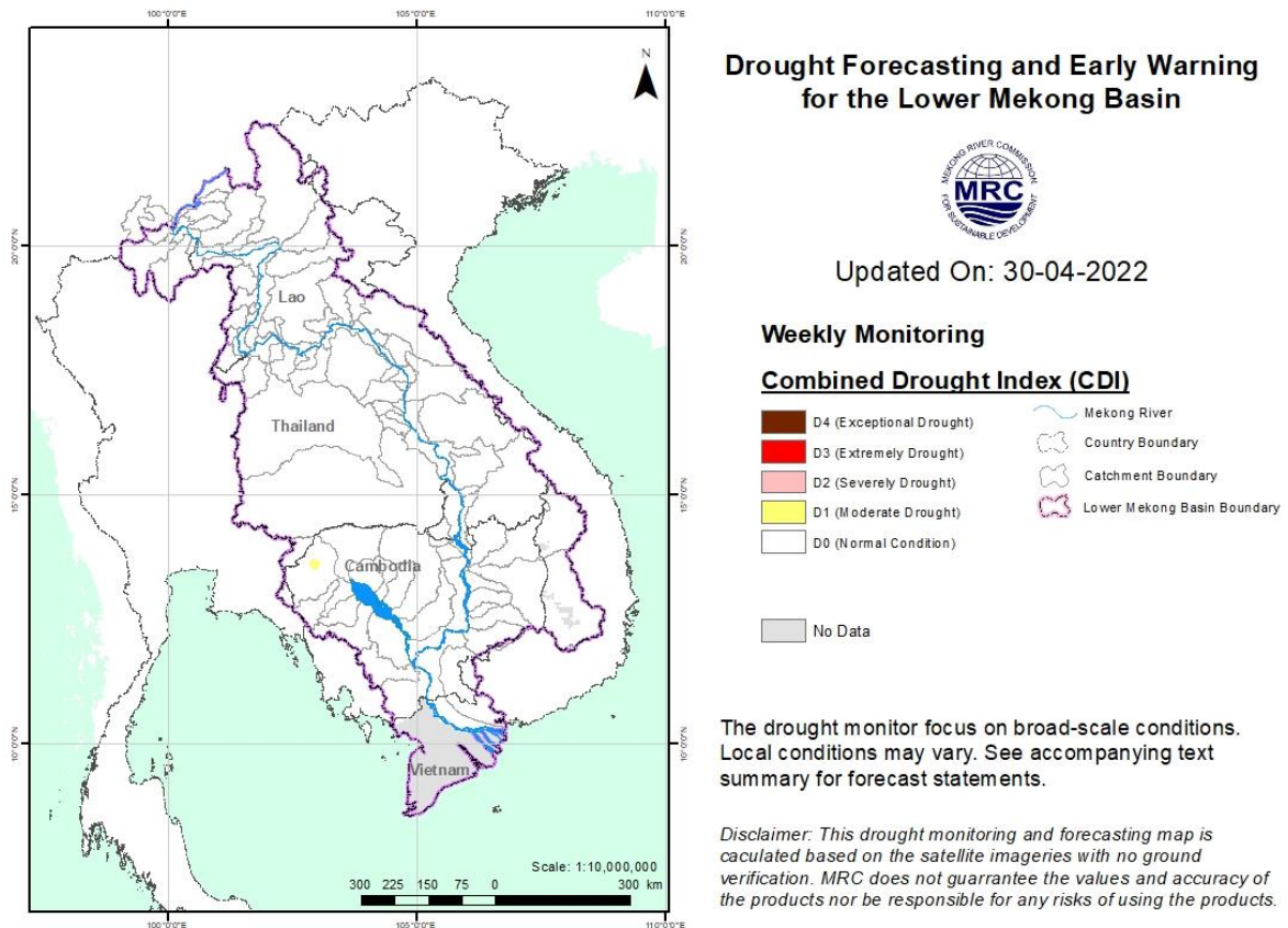
Figure 16: Weekly Combined Drought Index during April 24-30.
