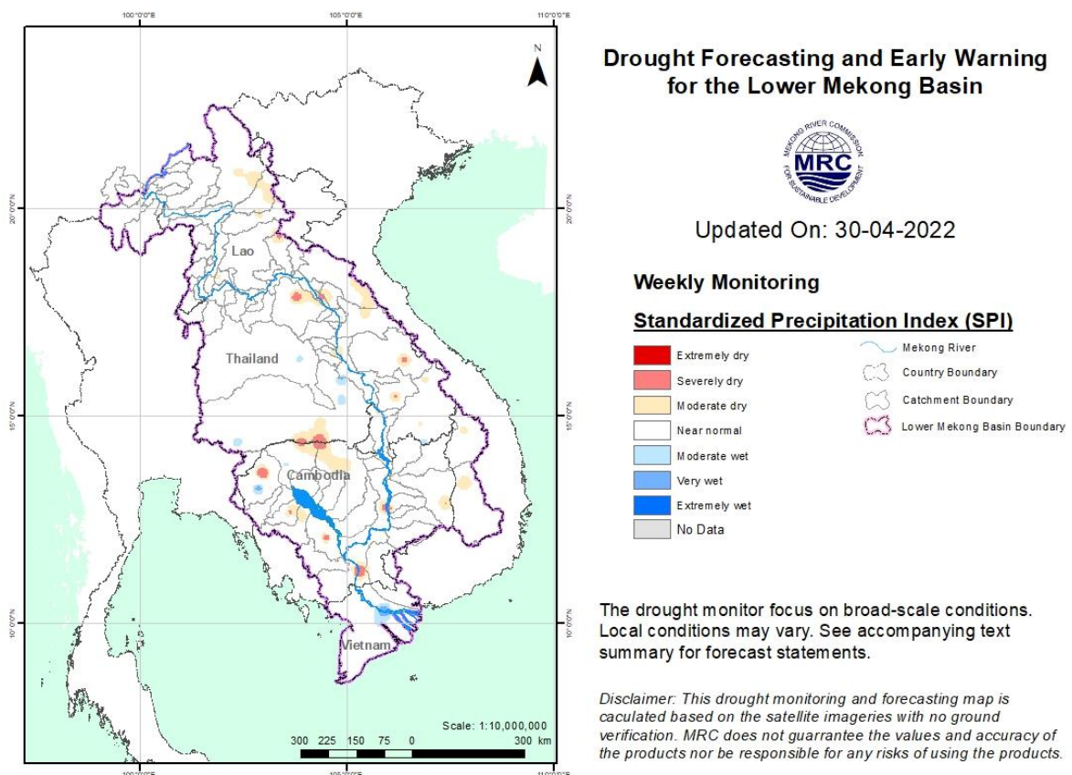
Figure 14: Weekly standardised precipitation index from April 24 to 30.
