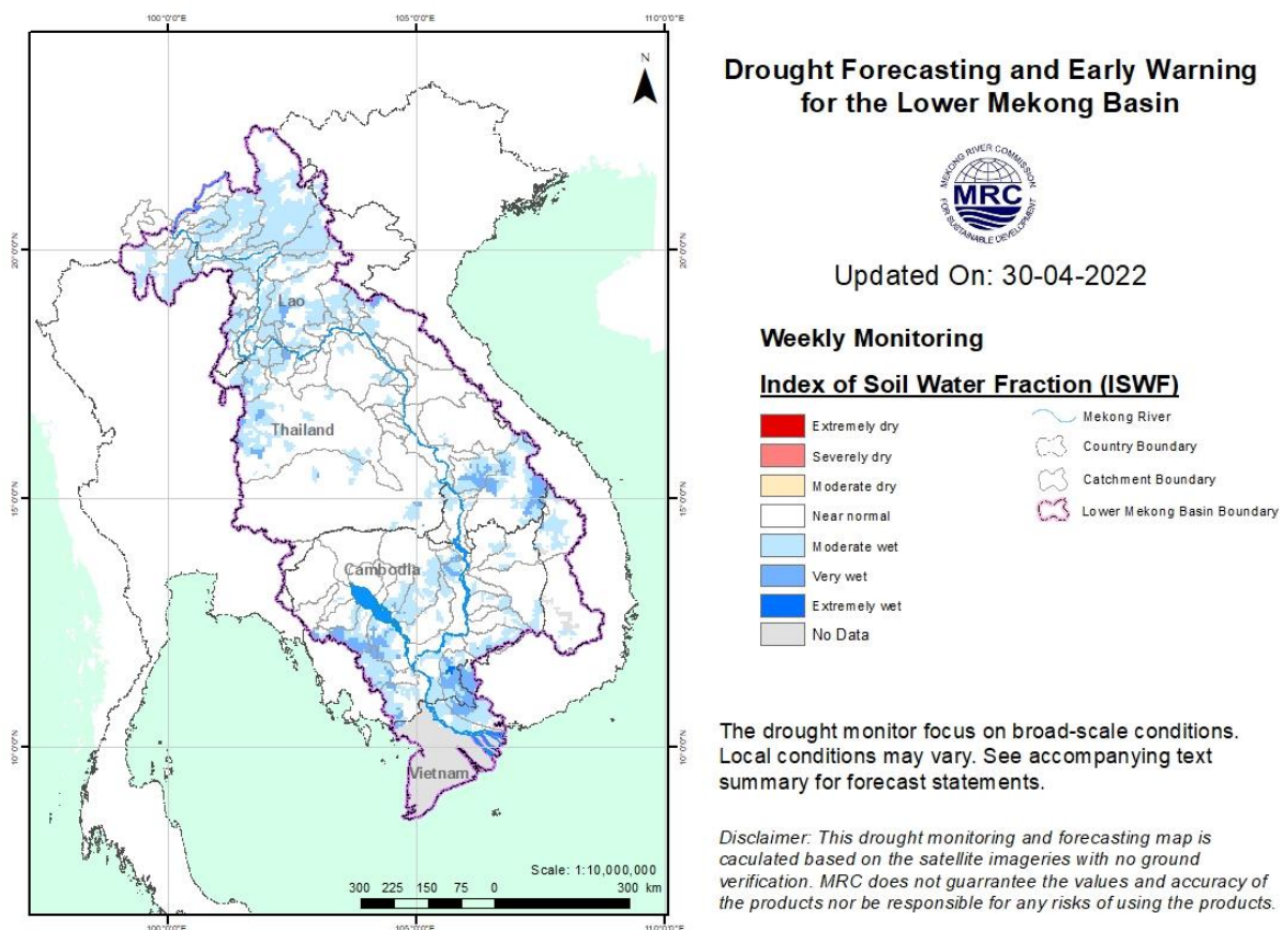
Figure 15: Weekly Index of Soil Water Fraction from April 24 to 30.
