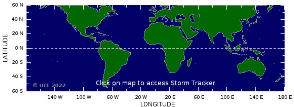
Figure 3: No tropical storm risk observed on 02 May 2022.
